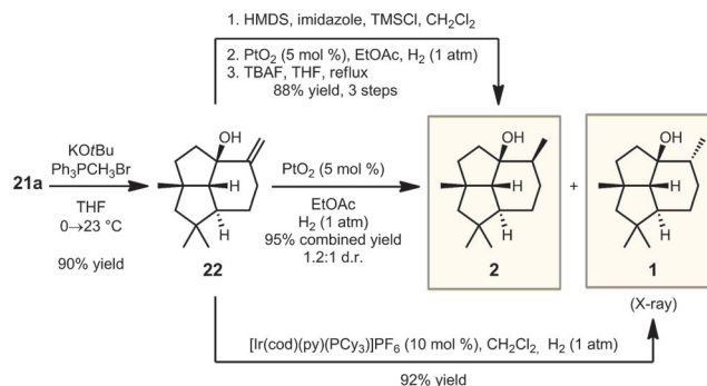
Scheme 3. Synthesis of the reported structures of 9- epi -presilpiperfolan-1-ol ( 2 ) and presilpiperfolan-1-ol ( 1 ).
