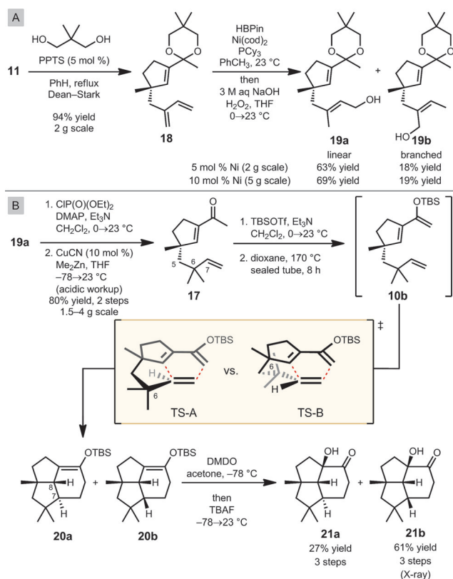
Scheme 2. Revised synthetic approach to presilpiperfolane core. cod = cyclooctadiene, DMAP = 4-dimethylaminopyridine, DMDO = dimethyldioxirane, TBAF = tetrabutylammonium fluoride.
